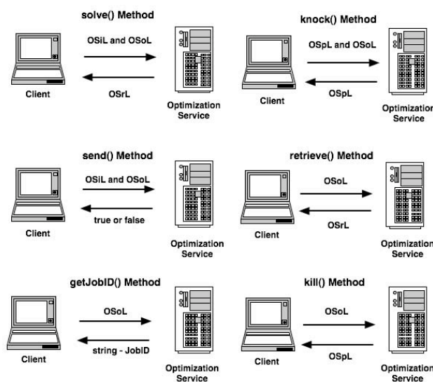
Figure 13 The OS hookup Language (OShL) communication methods.
