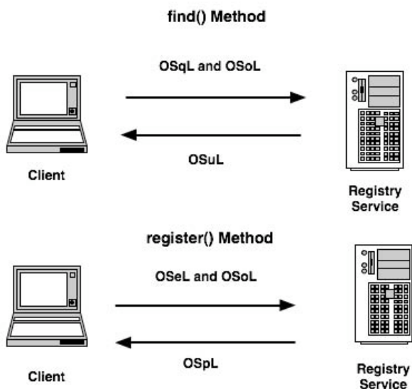
Figure 14 The OS discovery Language (OSdL) communication methods.
