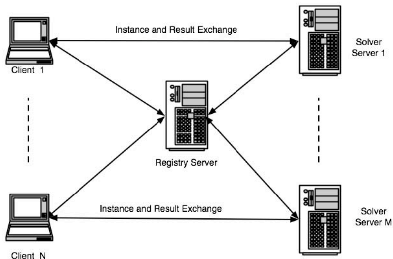
Figure 5 The Service Oriented Architecture version of Figure 3.
