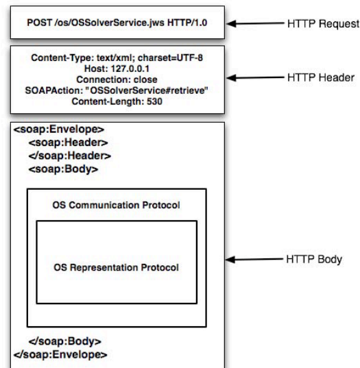
Figure 6 OS protocols inside a SOAP envelope inside an HTTP body.
